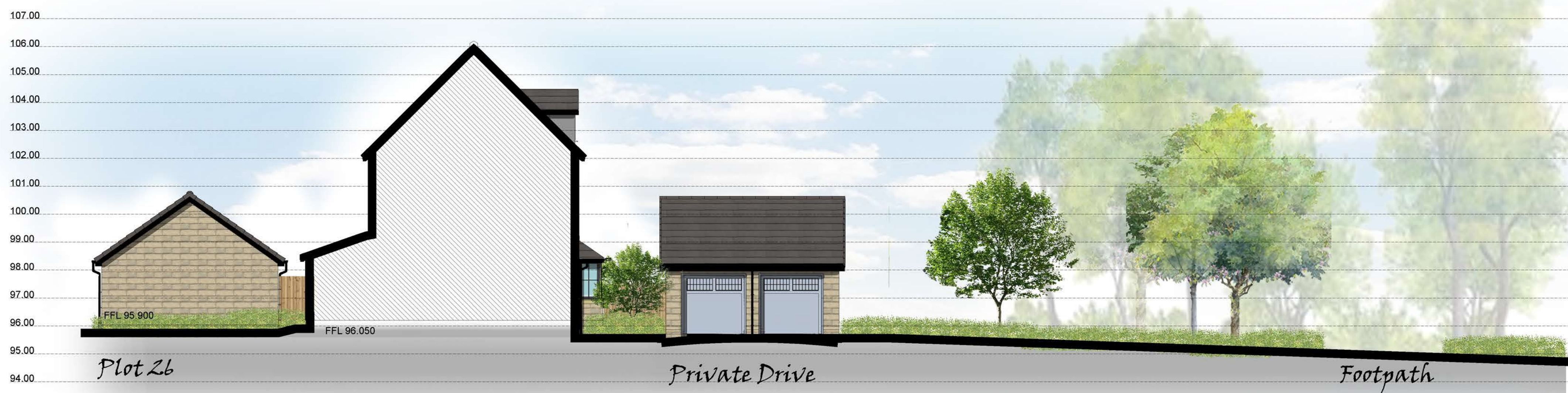
Cross Section X-X
