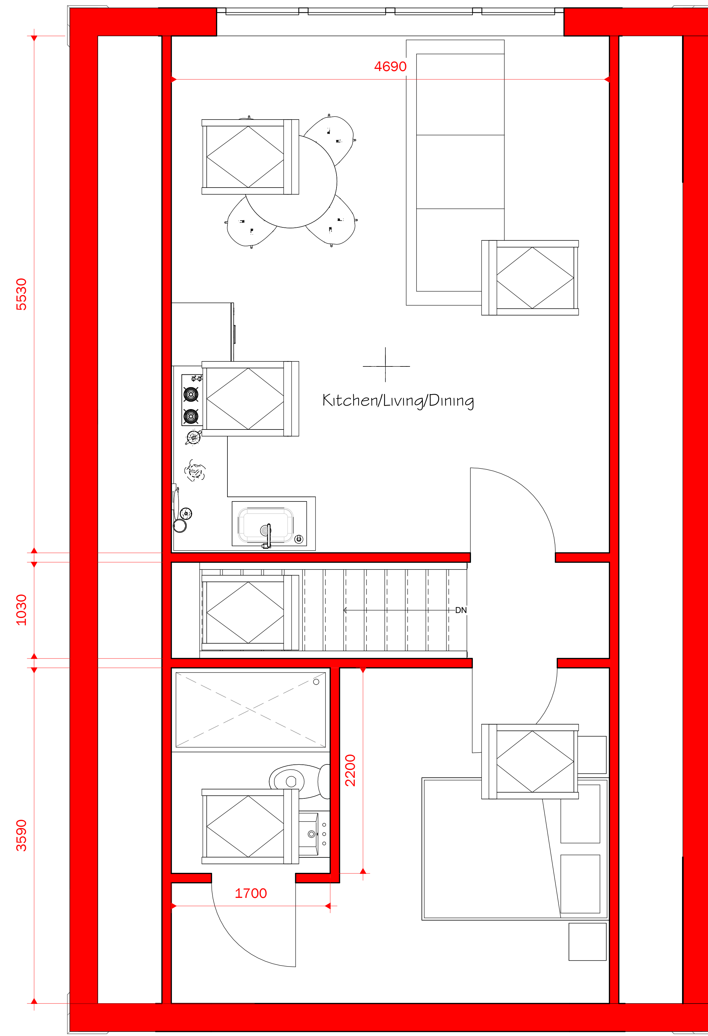
2 ANNEX PROPOSED FIRST FLOOR 1 : 25
