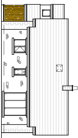
Proposed Front Elevation (Facing North)
