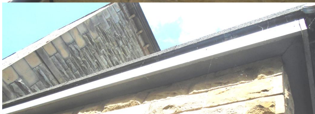
The eaves overhang is timber fascia boards and timber soffit. N.E.
