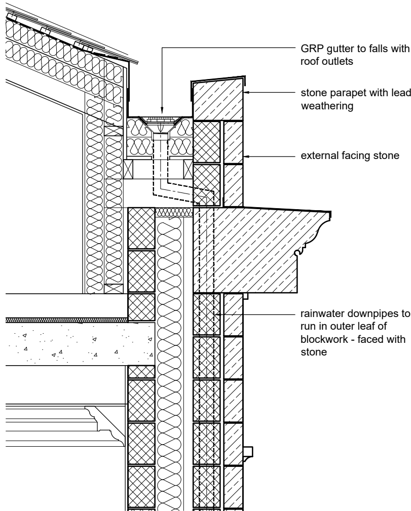
TYPICAL GUTTER DETAIL 1:20 scale
