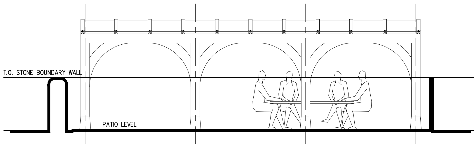
REAR ELEVATION.
