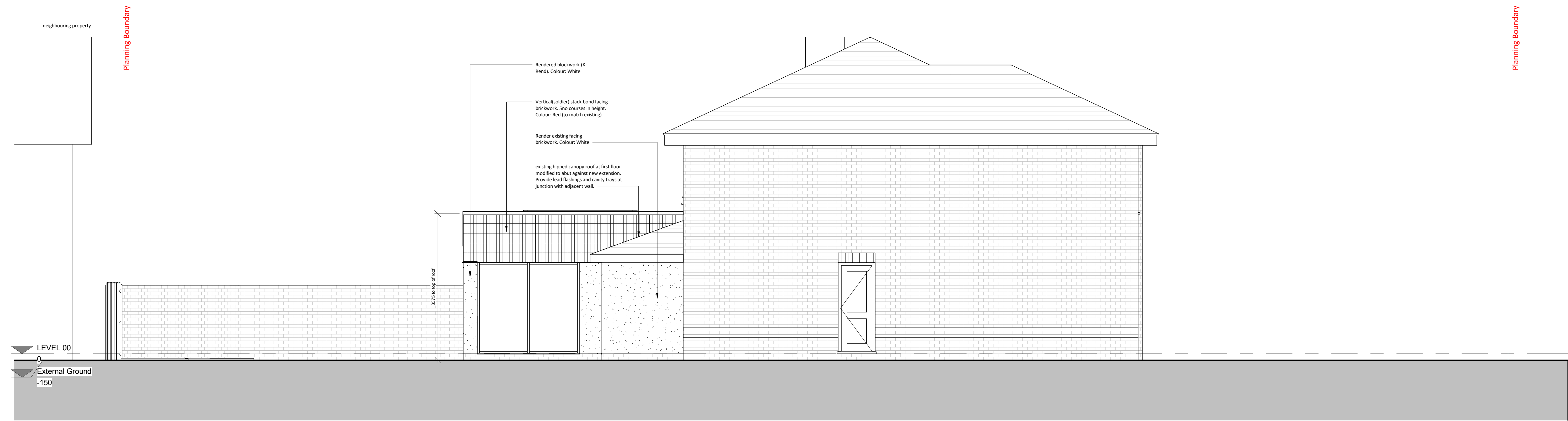
Side Elevation B - PROPOSED
