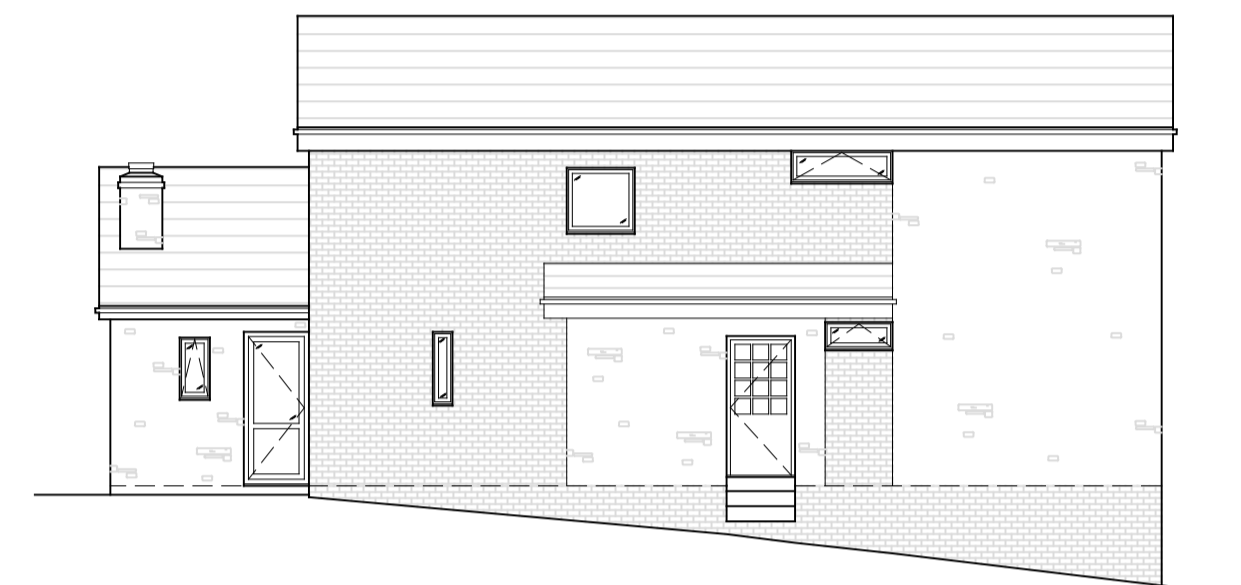
Side Elevation (Facing North)
