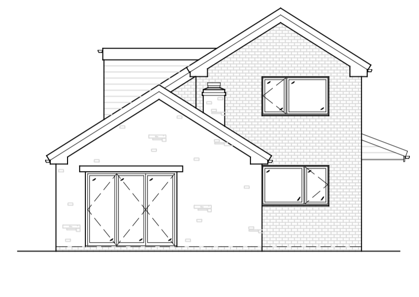
Rear Elevation (Facing East)
