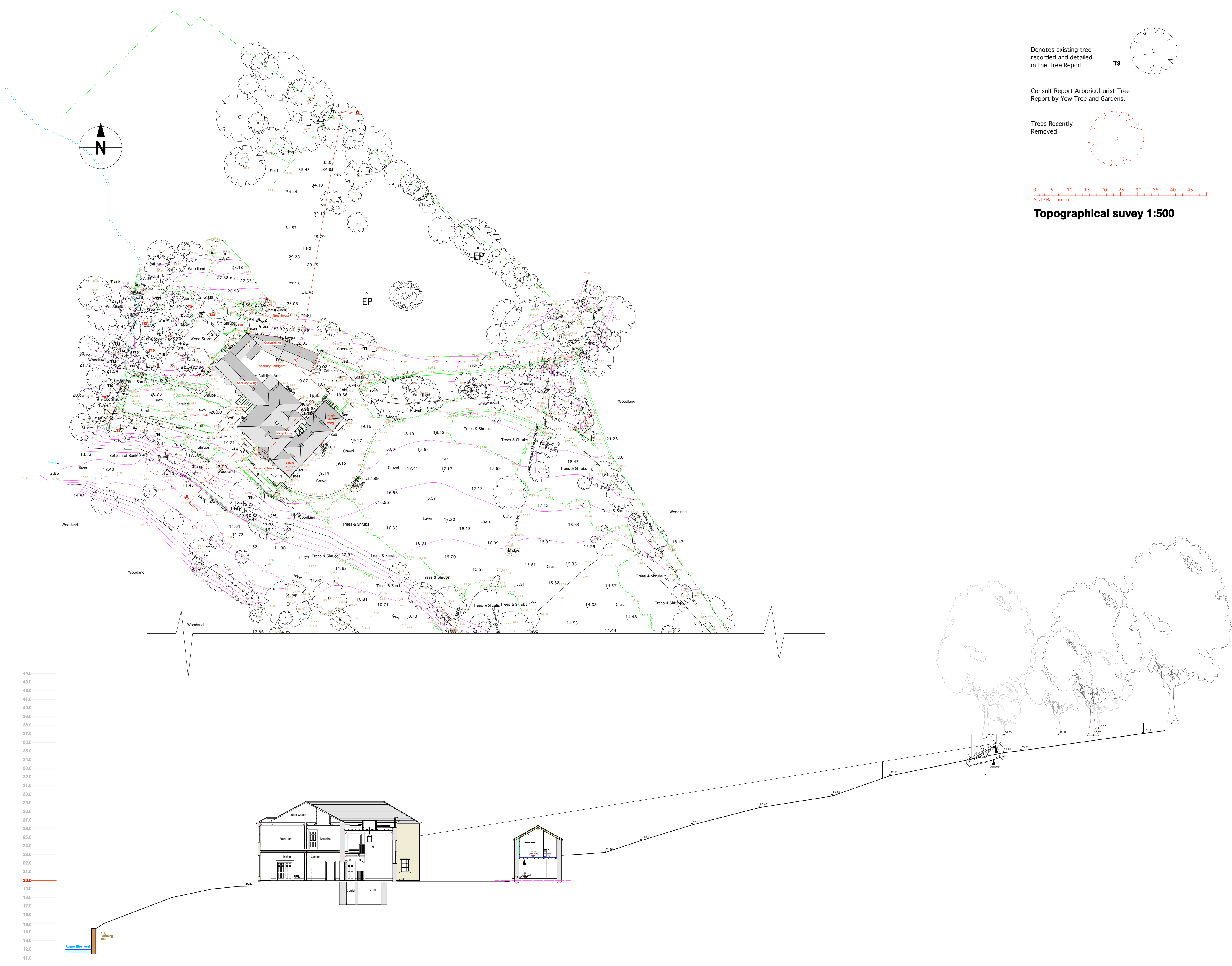
Section AA- extending up the hillside 1:200
