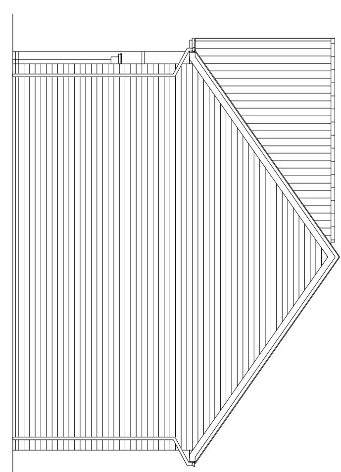
SIDE ELEVATION
