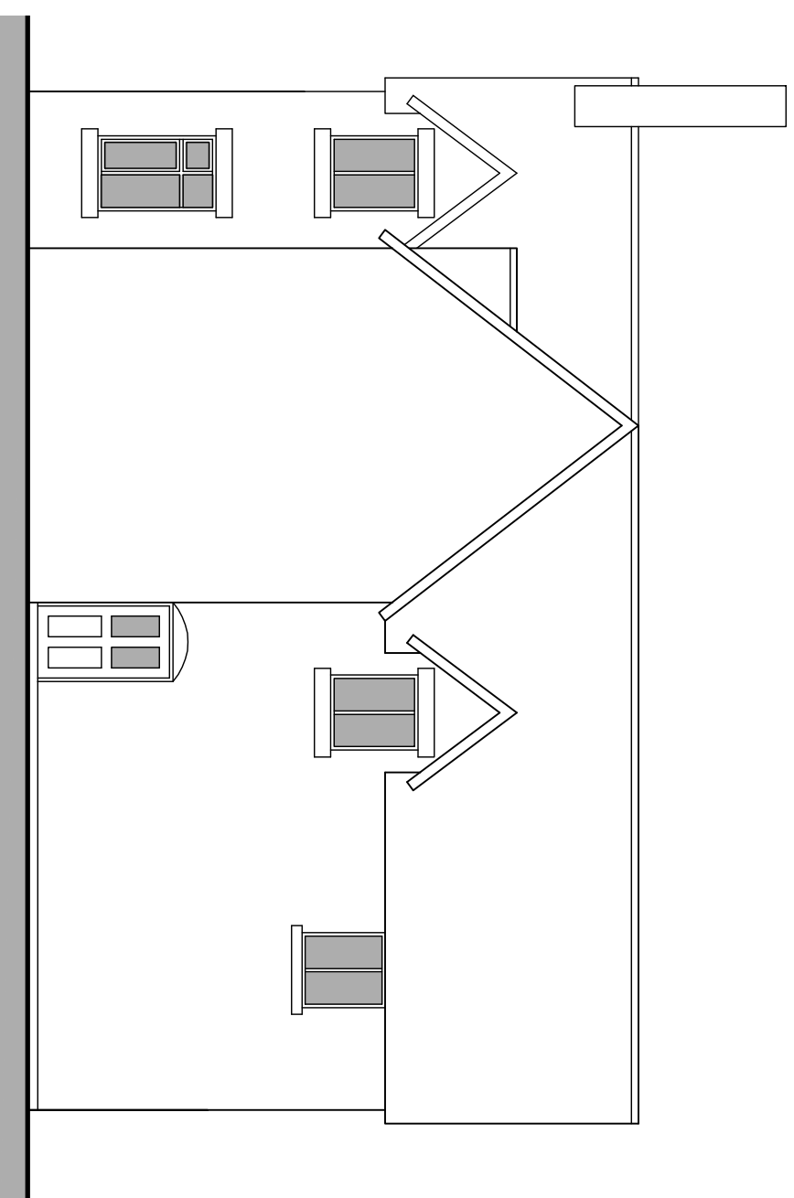
EXISTING ELEVATION 2 1:100
