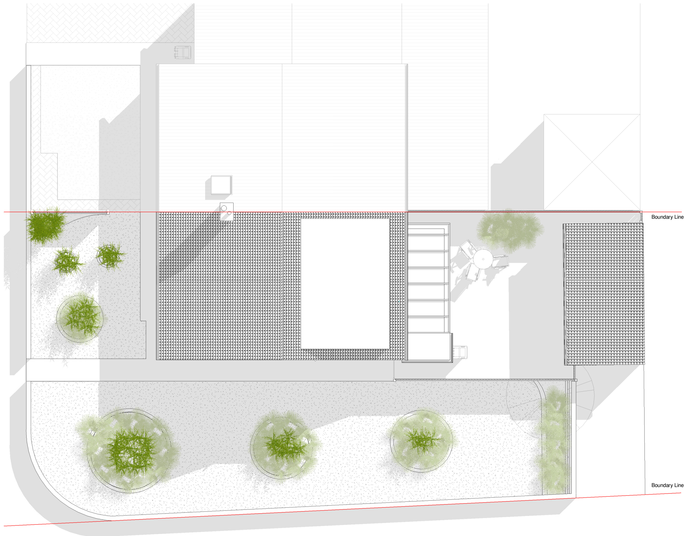
Roof plan.
