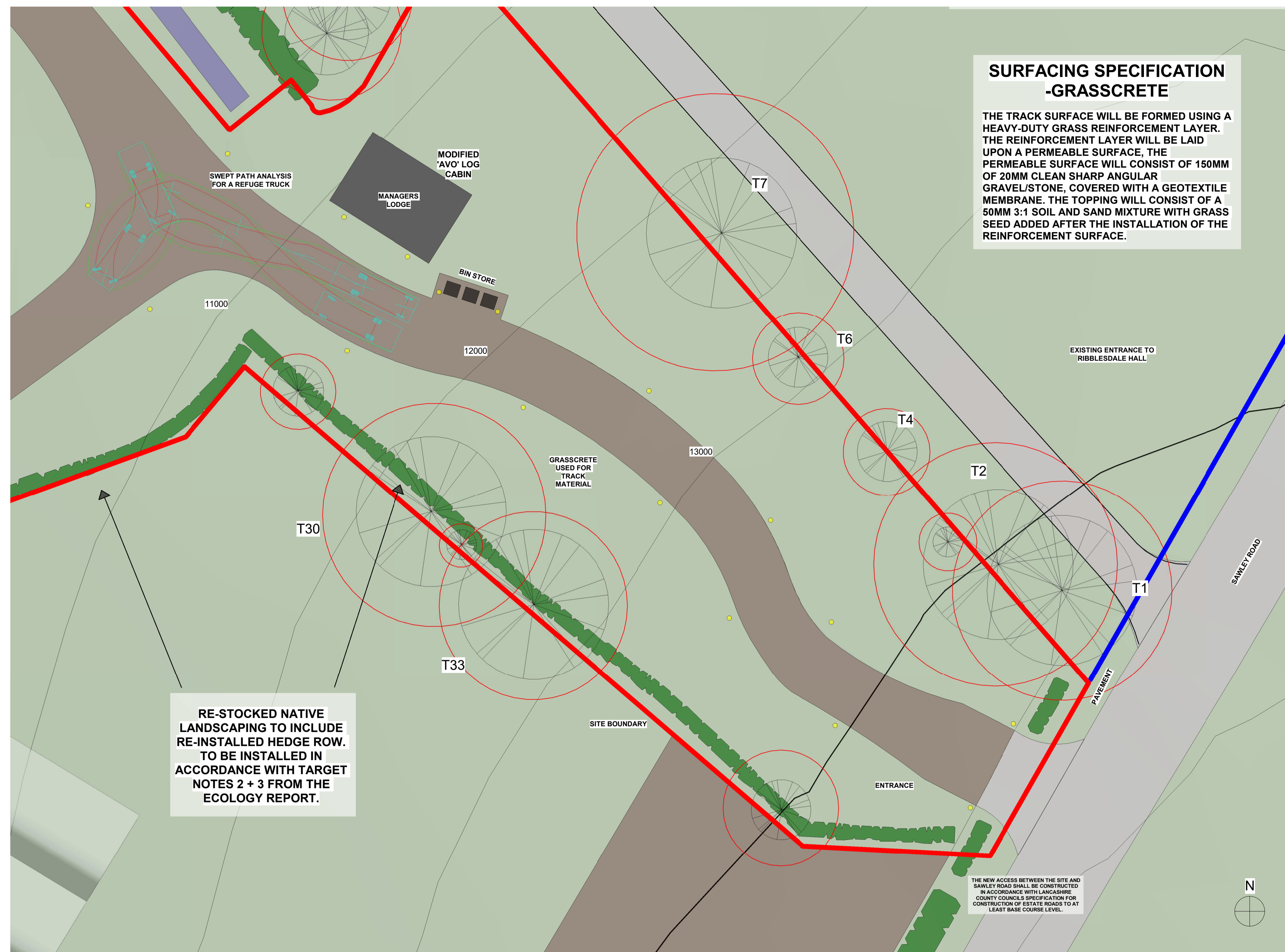
1 PROPOSED SITE PLAN DETAIL 1 : 200
