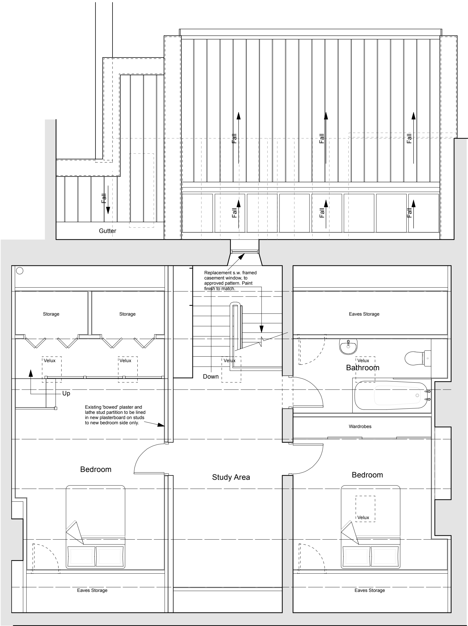
Second Floor Roofspace Plan
