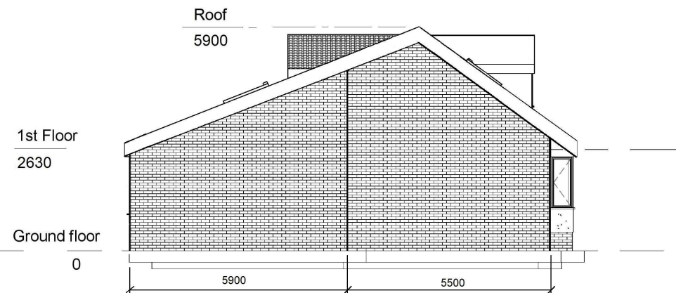
Proposed Side Elevation - LH (4)
