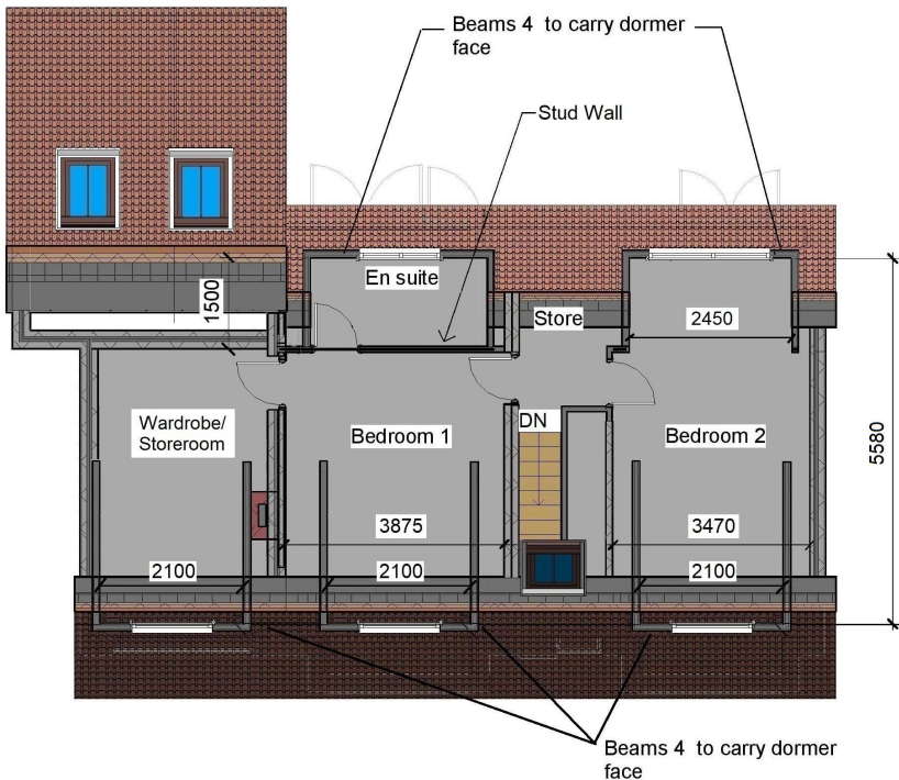
First Floor Section (2)
