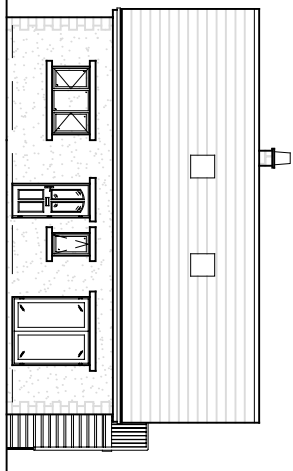
Proposed Rear Elevation (Facing South)
