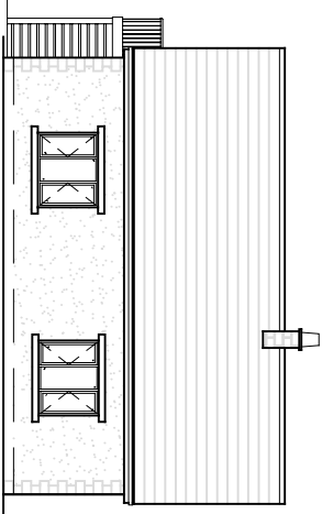
Proposed Front Elevation (Facing North)
