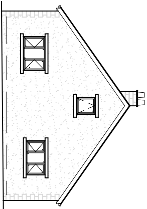
Proposed Side Elevation (Facing West)
