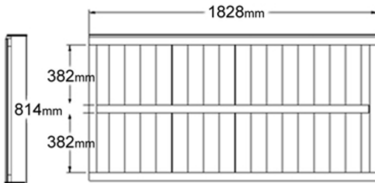
Panel Back
