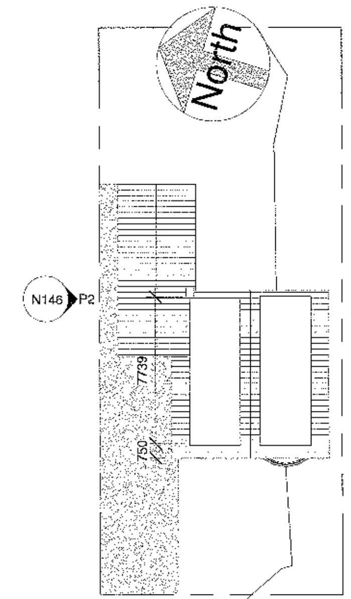
P6 Proposed Site Plan 1:200 N146
