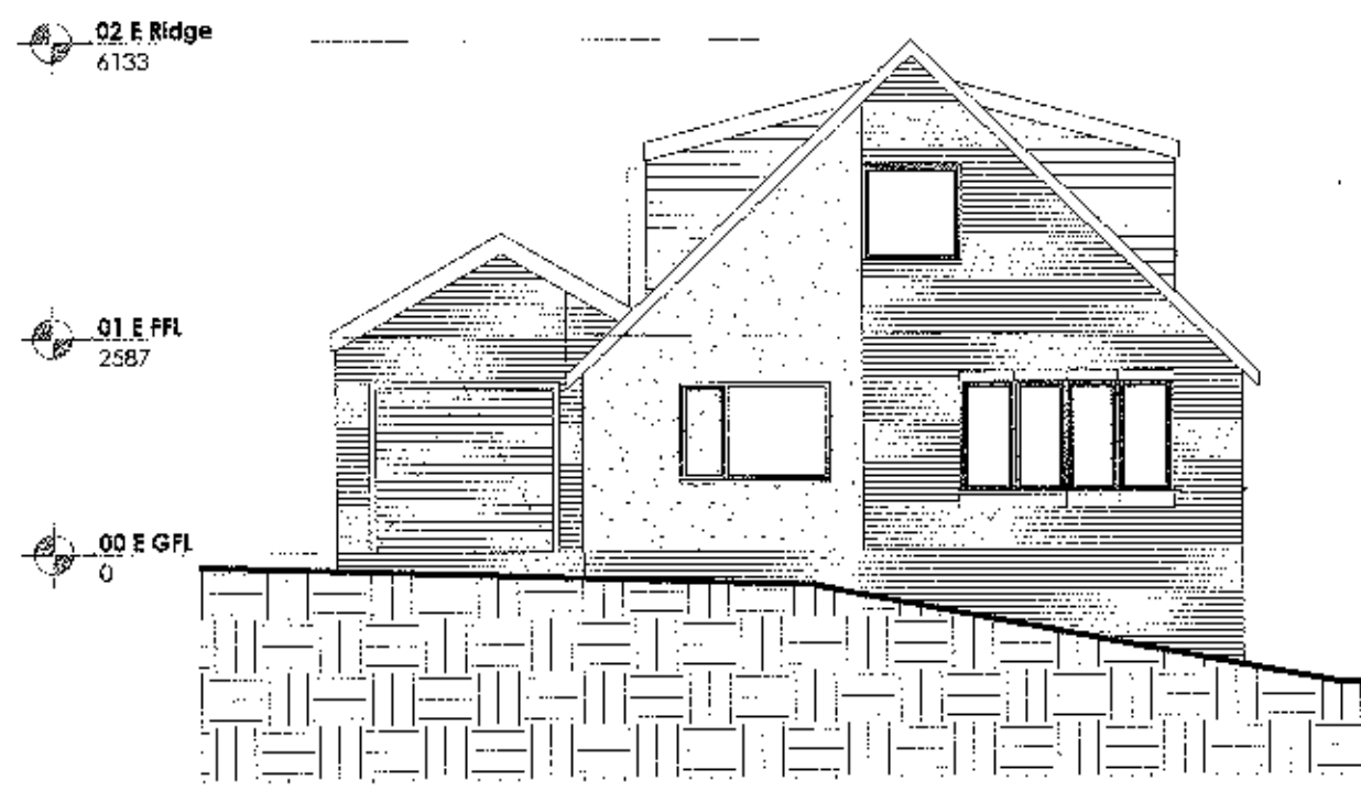
E1 Existing Front (W) Elevation 1:100 N146
