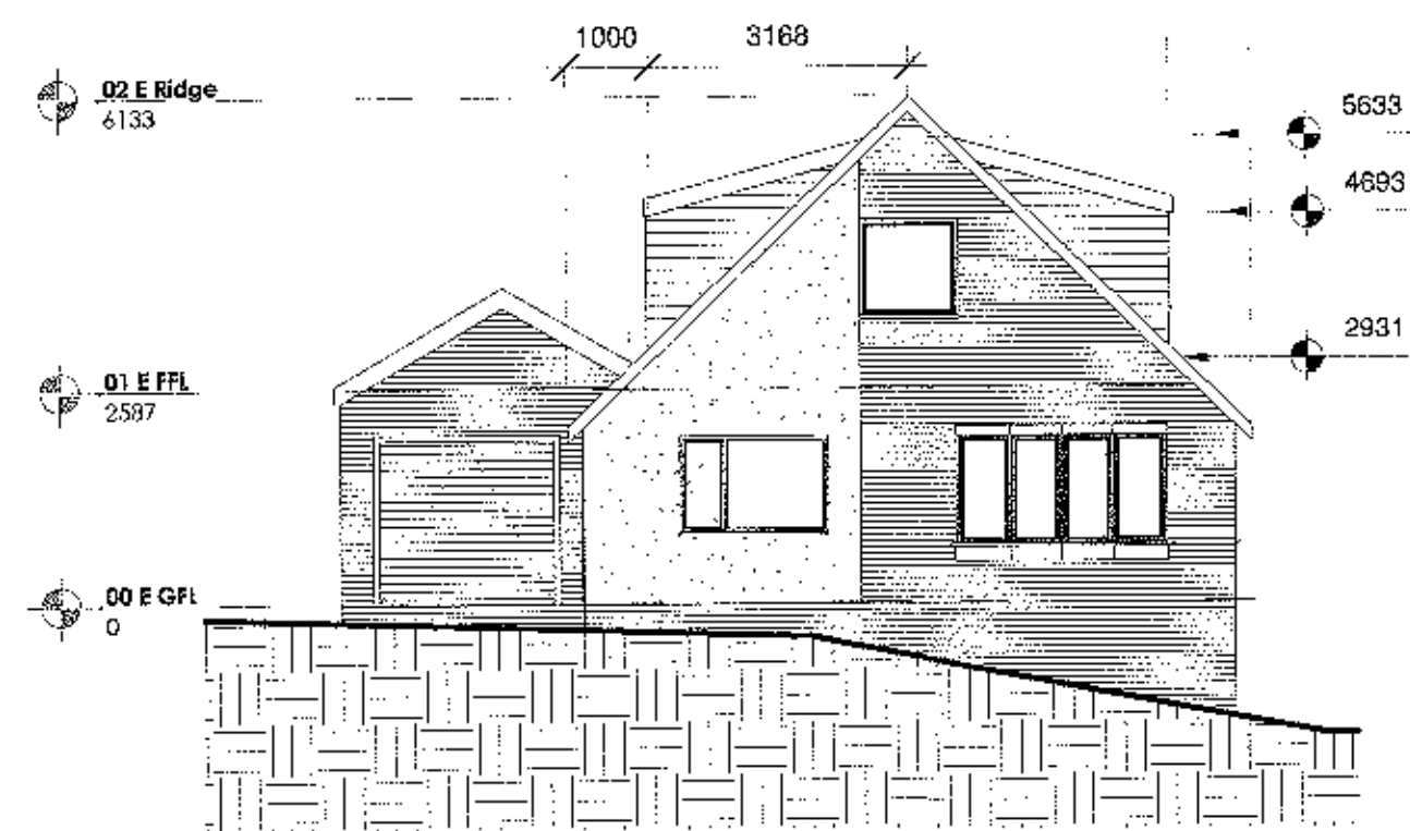
P1 Proposed Front (W) Elevation 1:100
