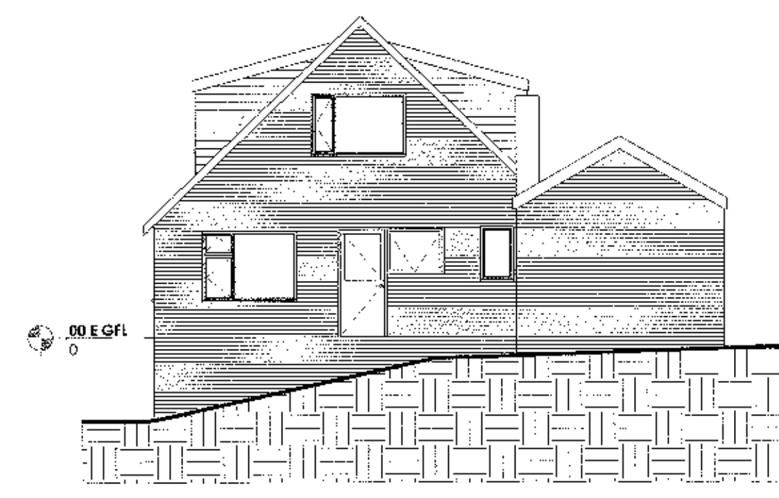
E3 Existing Rear (NE) Elevation 1:100 N146
