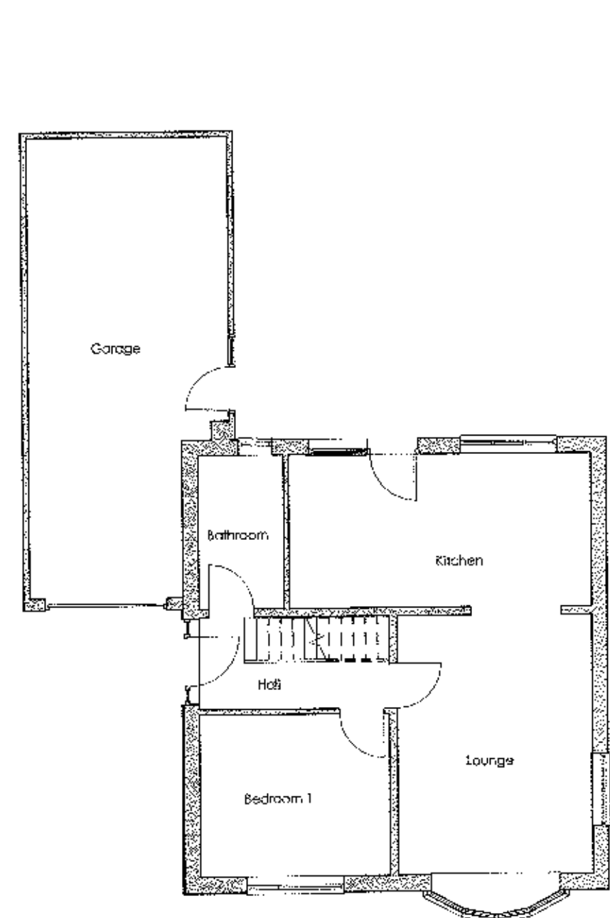
E5 Existing Ground Floor Plan 1:100 N146
