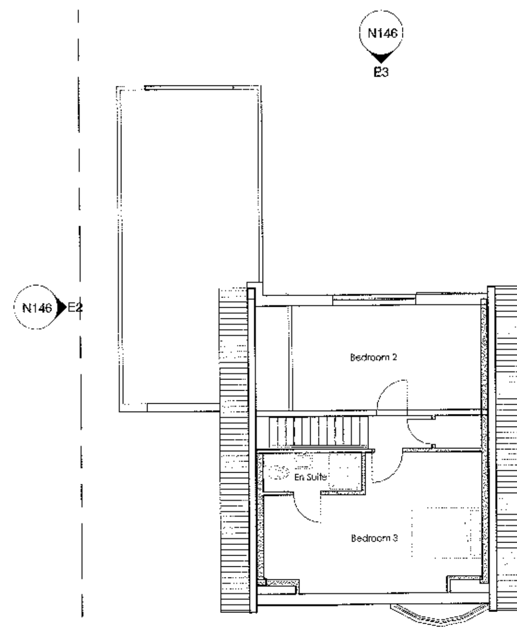
E6 Existing First Floor Plan 1:100 N146
