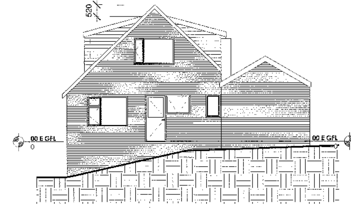
P3 Proposed Rear (NE) Elevation 1:100 N146
